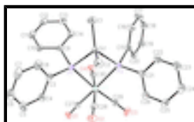
Fig. 1. The molecular structure of the title compound showing the atom-labelling scheme. H atoms are omitted for clarity. Displacement ellipsoids are drawn at the 30% probability level.
